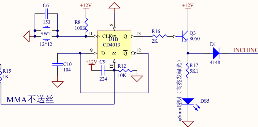
点动送丝
