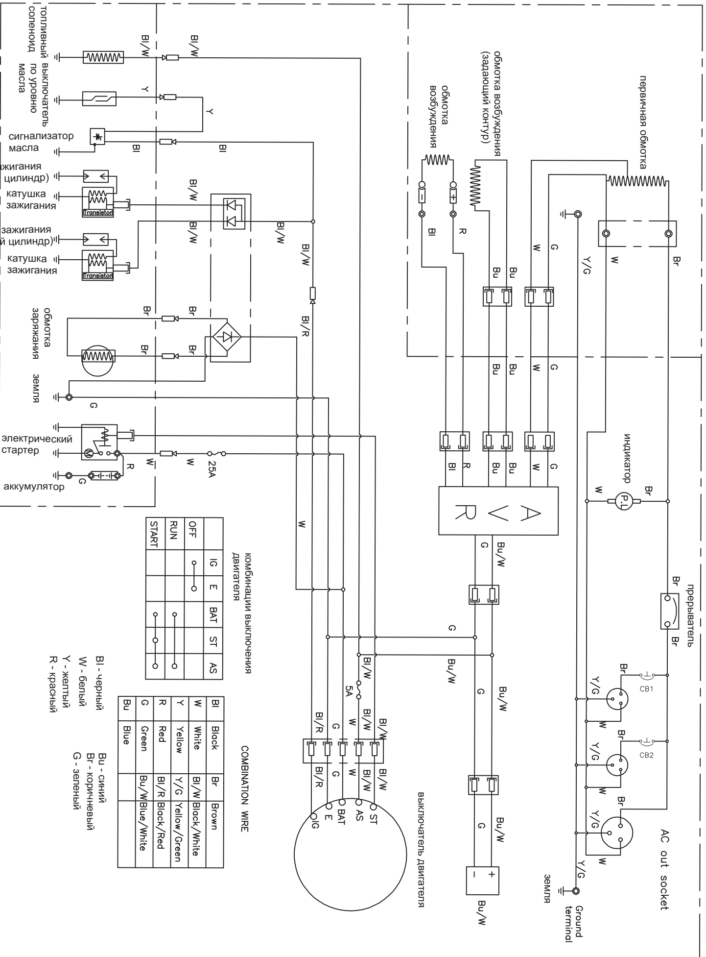
Engine block
